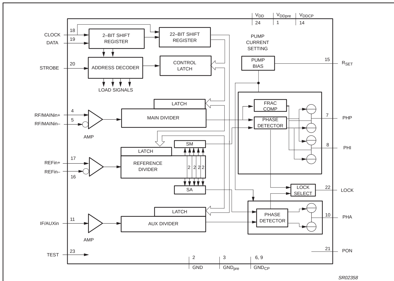
Figure 4. Block Diagram (HBCC24)
